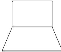
74280-L08 72" FIXTURE. ONE 48" SPACER AT THE MIDDLE OF THE TOTAL HEIGHT. SHOWN WITH A REC3-24 CANOPY.
