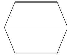
74280-L06 48" FIXTURE. ONE 72" SPACER AT THE MIDDLE OF THE TOTAL HEIGHT. SHOWN WITH A REC4-48 CANOPY.
