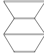
74280-L03 24" FIXTURE. ONE 48" SPACER AT THE FIRST THIRD AND ONE 24" SPACER AT THE SECOND THIRD. SHOWN WITH A REC4-48 CANOPY.
