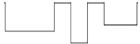
74280-L12 ONE 24" FIXTURE, ONE 48" FIXTURE AT THE MIDDLE OF THE TOTAL HEIGHT AND ONE 72" FIXTURE AT THE FIRST THIRD OF THE TOTAL HEIGHT. SHOWN WITH THE REC8 CANOPY OPTION AND A 192" TOTAL WIDTH.
