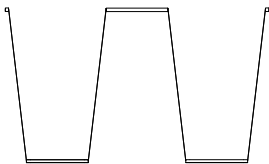
74280-L10 24" FIXTURES WITH TWO ANCHORS. SHOWN WITH THE REC8 CANOPY OPTION AND A 108" TOTAL WIDTH.
